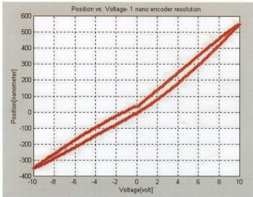
Figure 9: Typical DC Mode Behaviour
