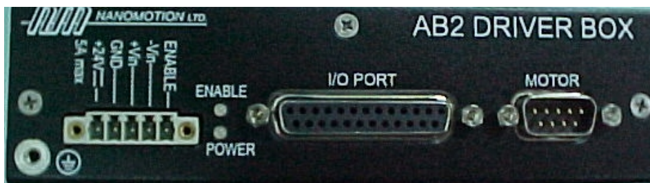
Figure 3: AB2 Driver Box Front Panel
