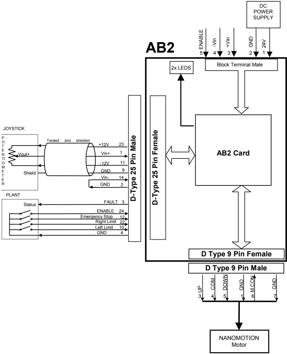
Figure 6: Joystick Connection
